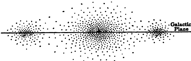
FIG. 1.—Hypothetical Section of the Stellar System.
